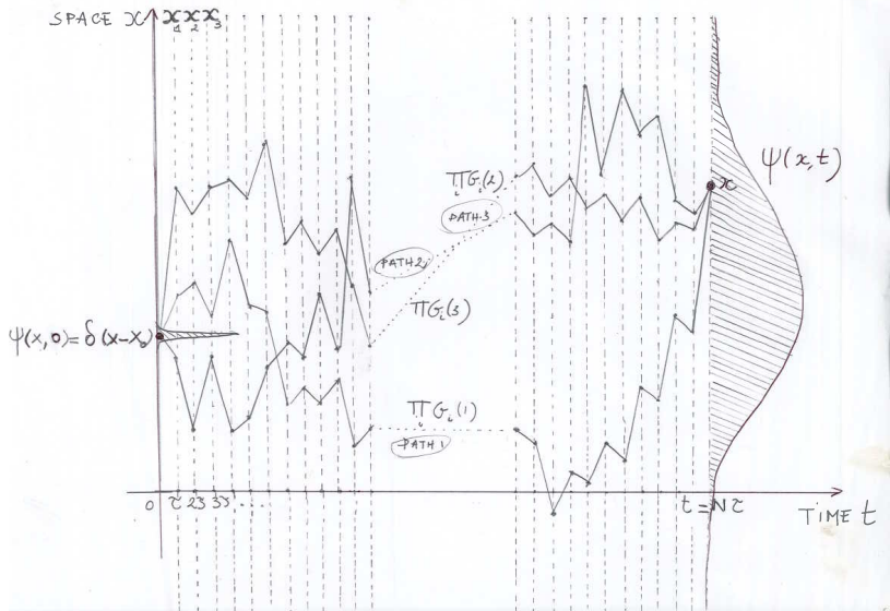
Figure: Pictorial representation of the sum over paths
