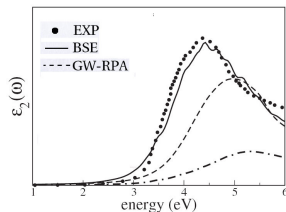
Silicon nanowire
