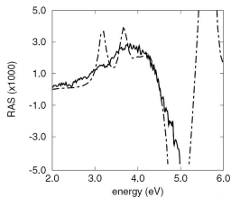
Diamond(100)(2x1)
